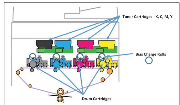
Bias Charge Rolls generate a uniform electrical charge across the Drum Cartridges, which produces smoother halftones than other technology.
